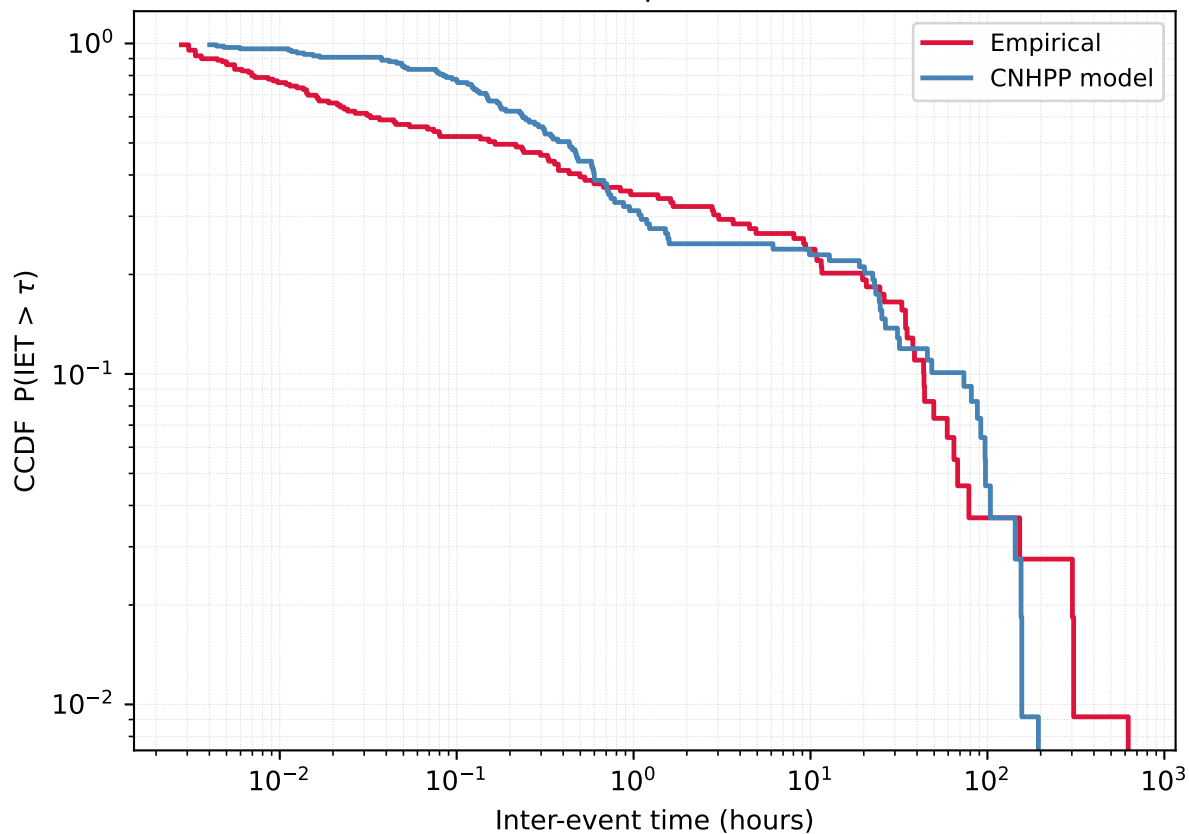
User 882741473 - Empirical vs CNHPP model
