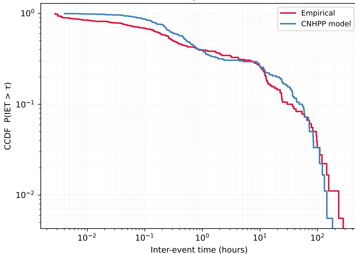
User 53034376 - Empirical vs CNHPP model
