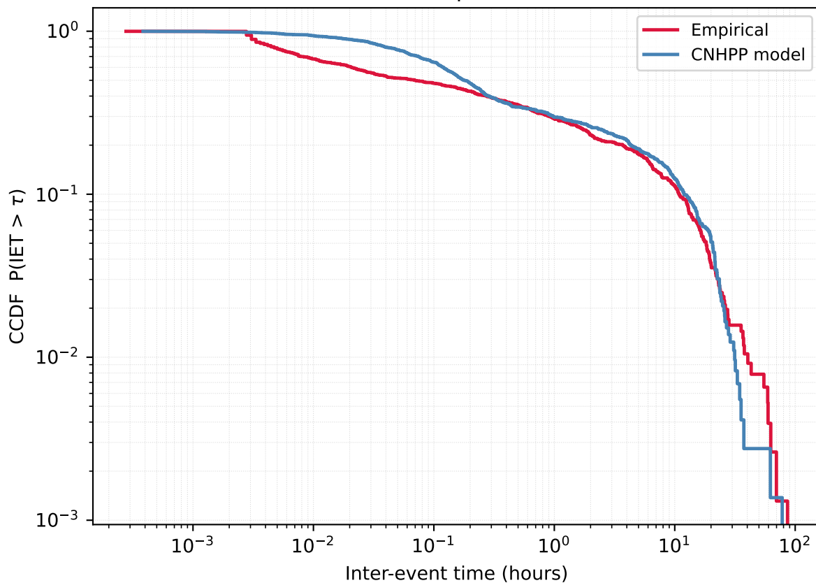
User 8336493019 - Empirical vs CNHPP model
