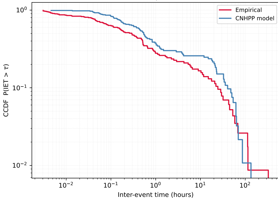
User 1083421726 - Empirical vs CNHPP model
