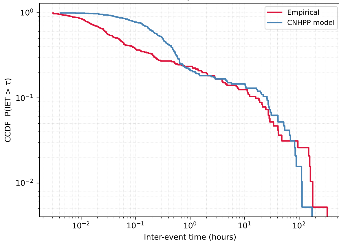
User 698141415 - Empirical vs CNHPP model
