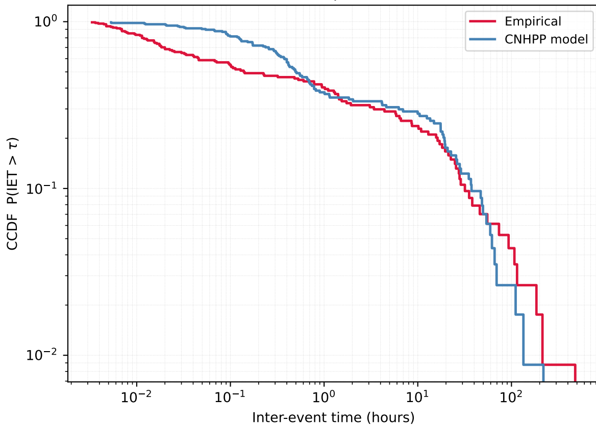
User 1753465784 - Empirical vs CNHPP model
