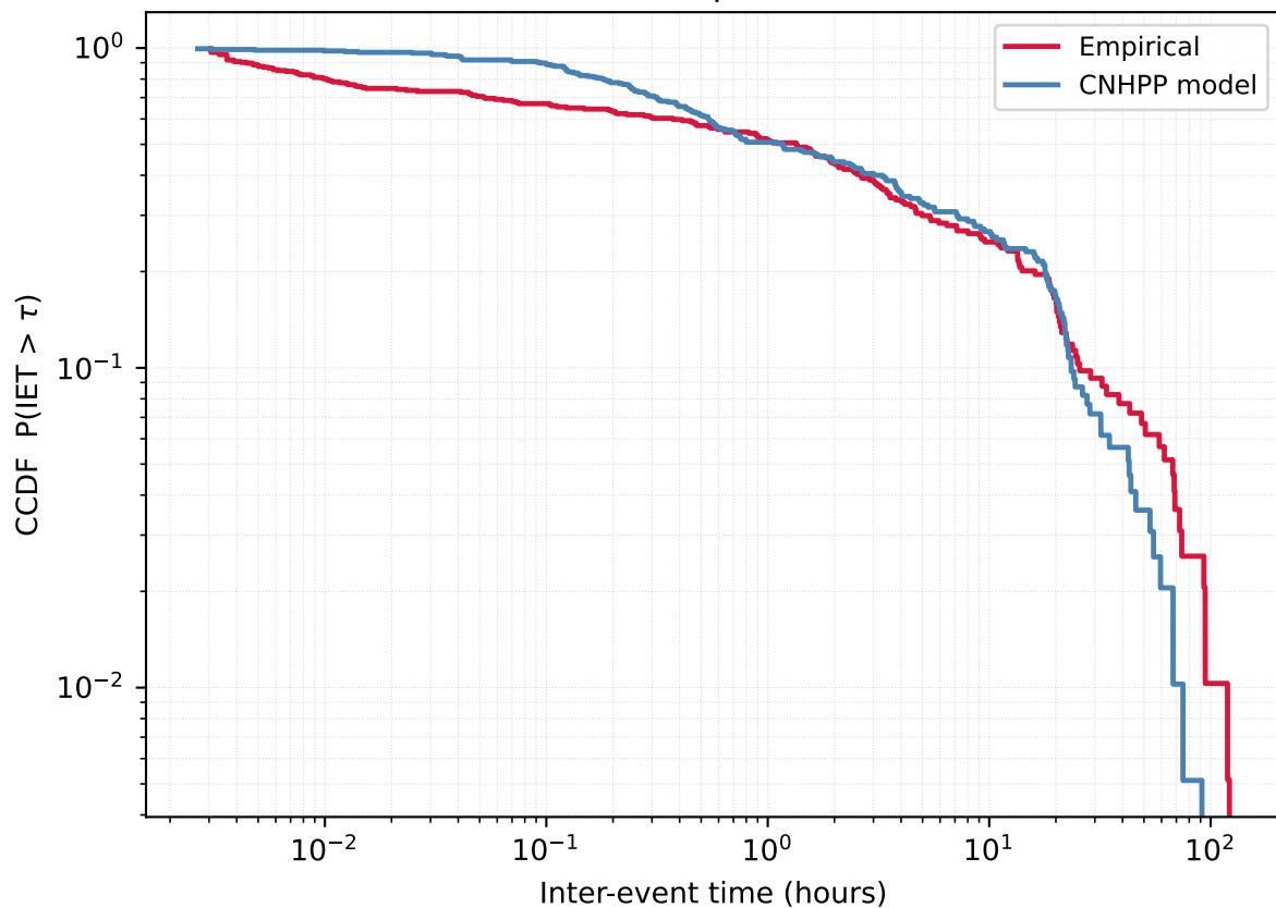
User 6111348138 - Empirical vs CNHPP model
