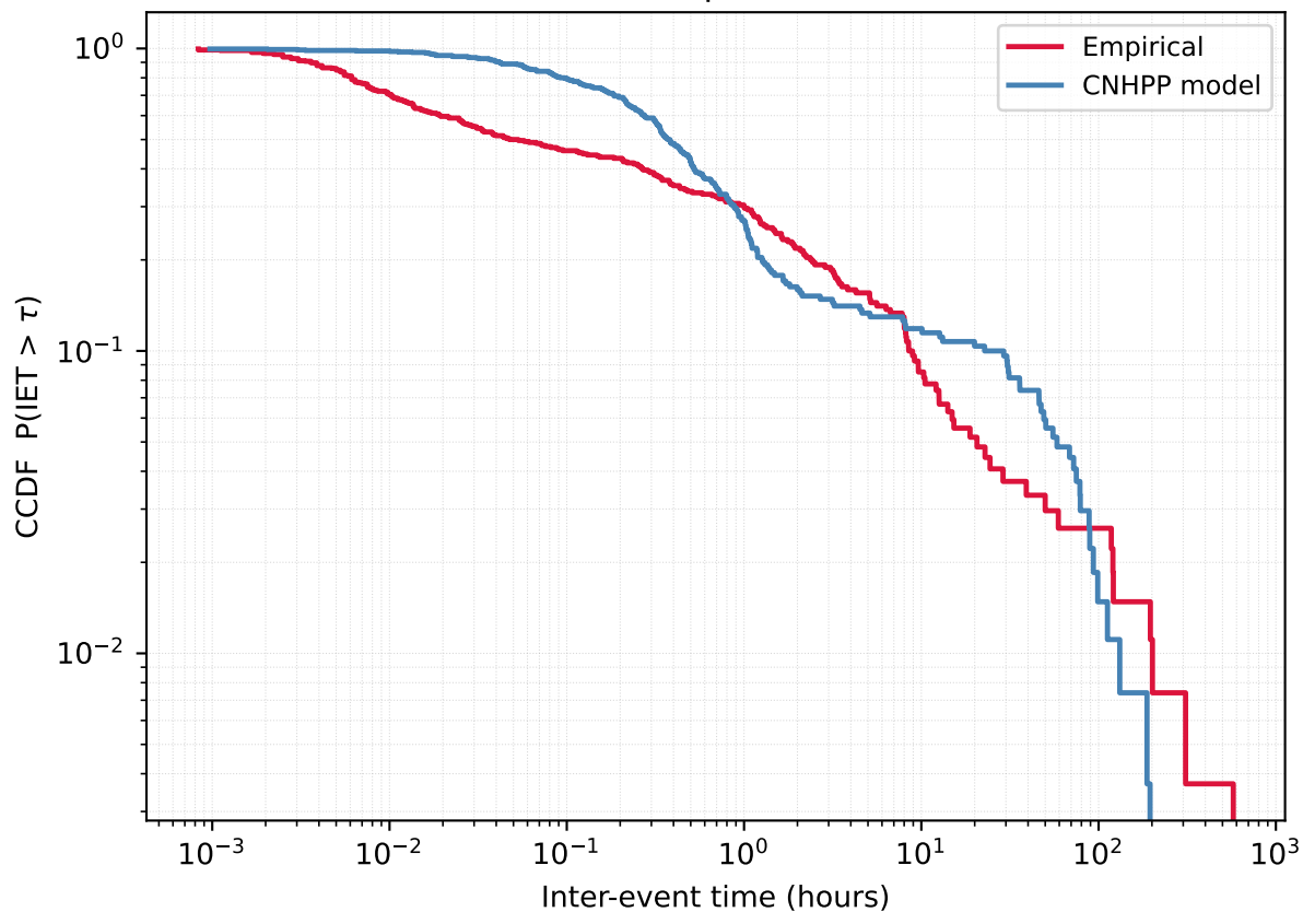
User 145800528 - Empirical vs CNHPP model
