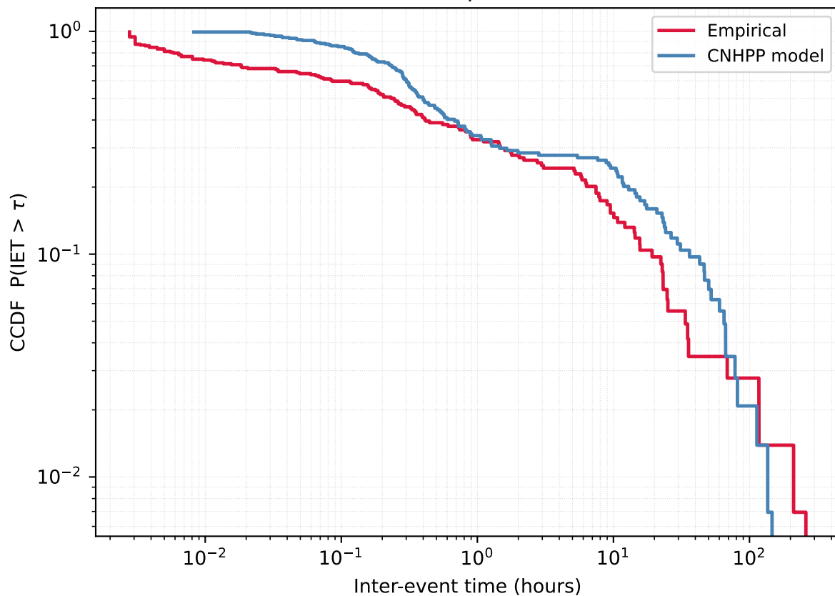
User 5213718005 - Empirical vs CNHPP model
