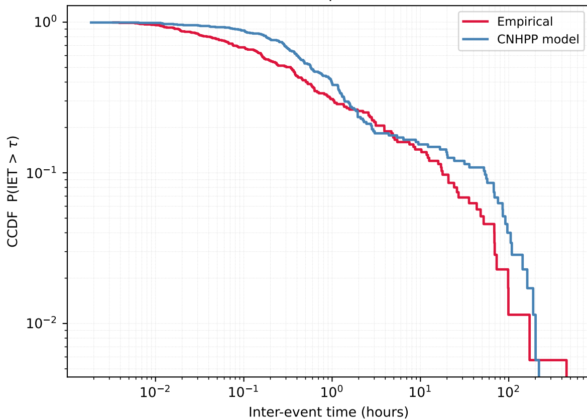
User 6947363606 - Empirical vs CNHPP model
