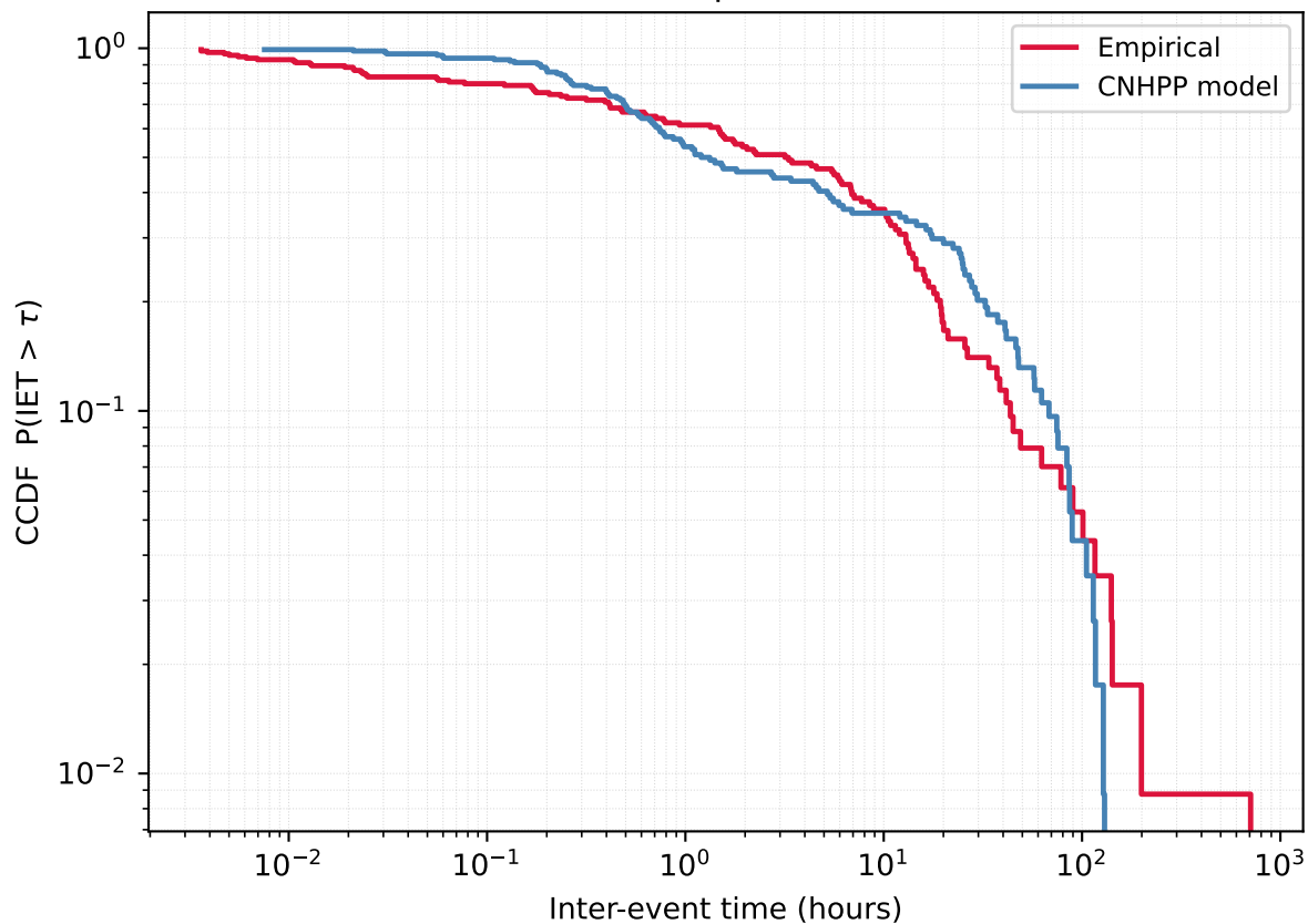
User 405690380 - Empirical vs CNHPP model
