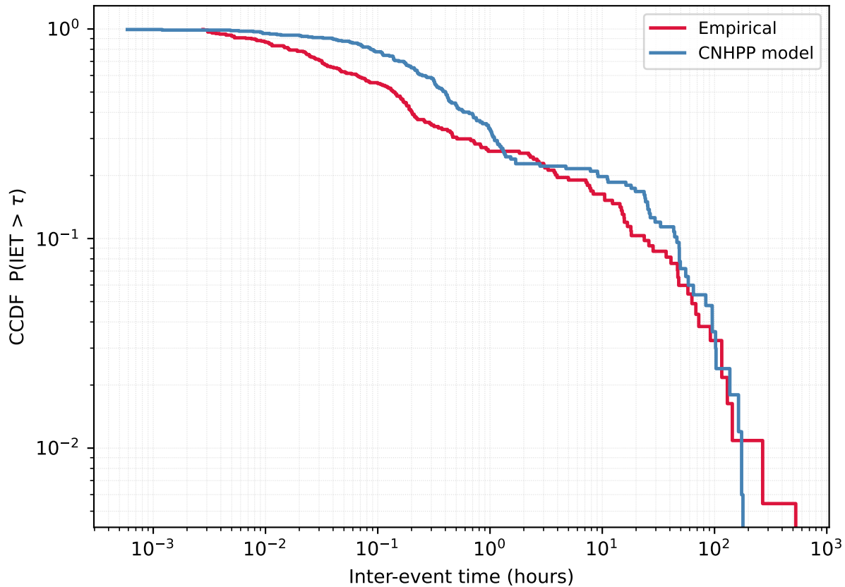
User 17798588 - Empirical vs CNHPP model
