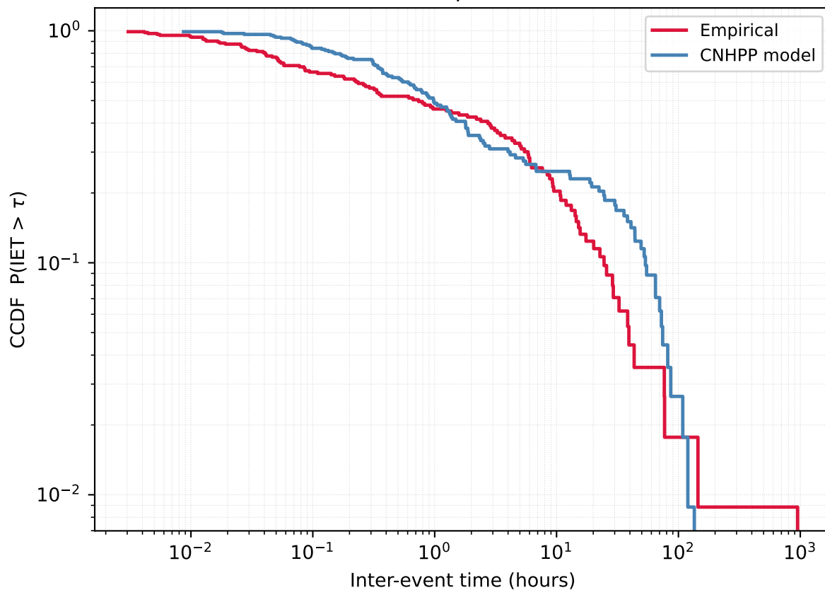
User 459294324 - Empirical vs CNHPP model
