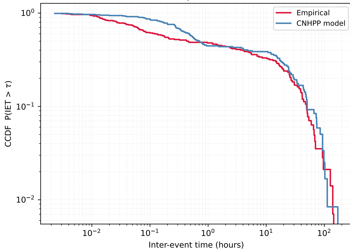
User 7678561 - Empirical vs CNHPP model
