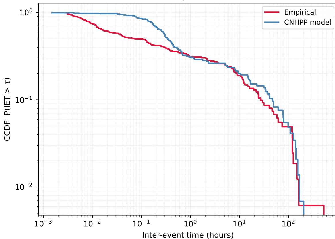
User 36162471 - Empirical vs CNHPP model
