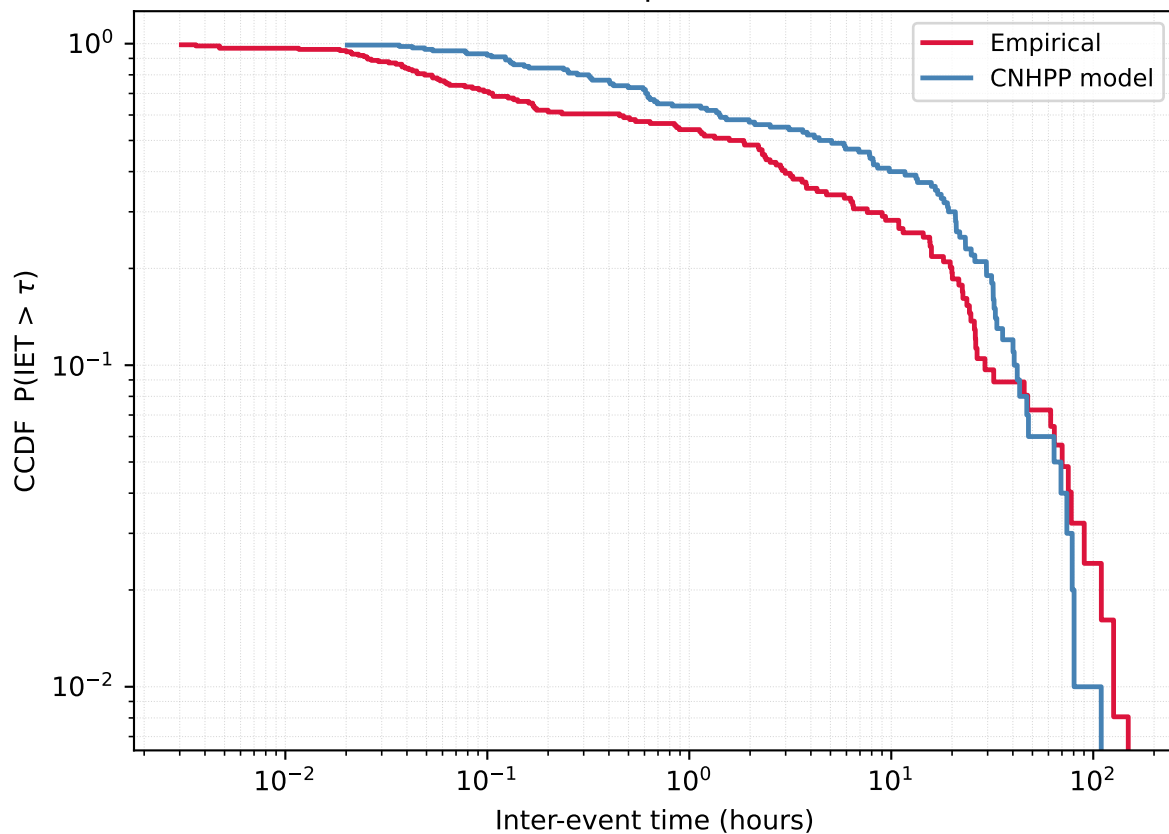
User 458678536 - Empirical vs CNHPP model
